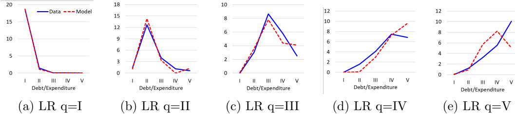
Figure 3: Joint Leverage Ratio and Debt-to-Expenditure Ratio Distribution
